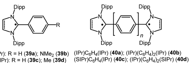
Fig. 10 NHC stabilized radicals over extended carbon systems.
