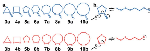
Scheme 1 (a) Series of cyclic thiosulfates and cyclic disulfides examined in this manuscript. (b) Mechanism of thiol-disulfide exchange between nucleophilic methyl thiolate ( \text{MeS}^- ) and a cyclic thiosulfate (blue) or a cyclic disulfide (red).
