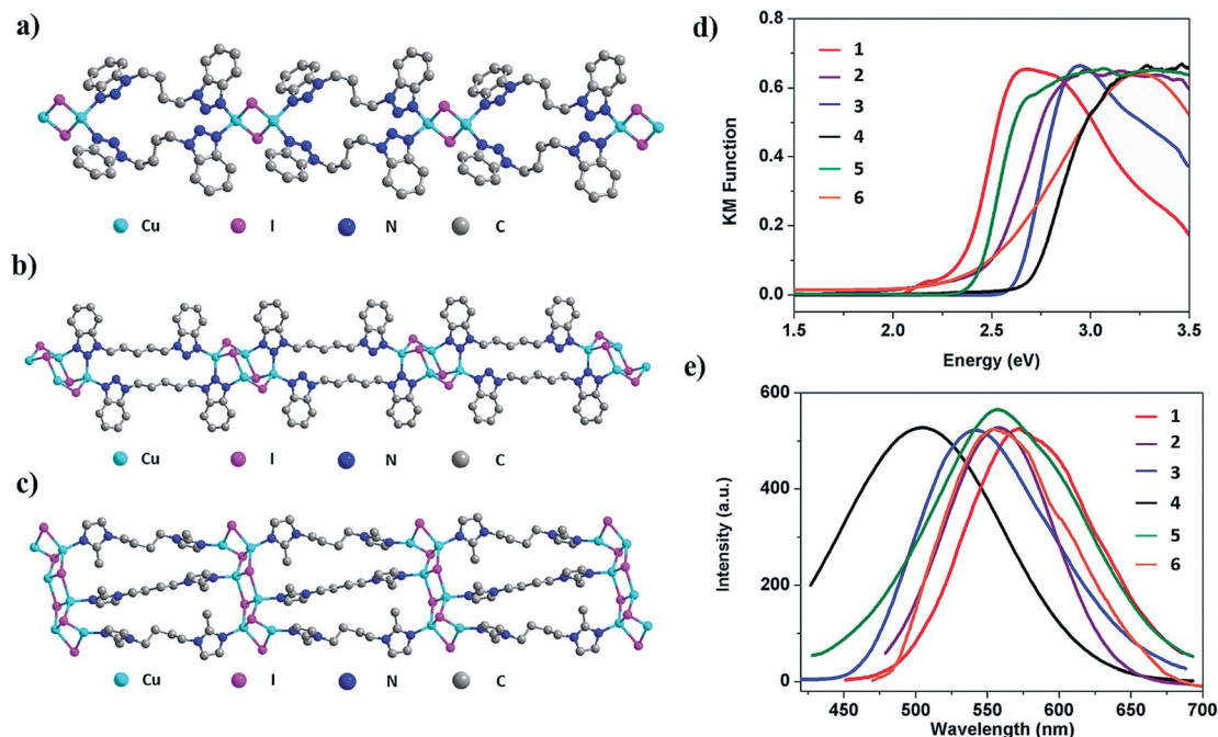
Fig. 2 (a) 1D-Cu 2 I 2 (bbt 2 bu) 2 (2). (b) 1D-Cu 4 I 4 (bbtpe) 2 (5). (c) 1D-Cu 6 I 6 (bmibu) 3 (6). Color scheme of the atoms: Cu: cyan, I: pink, N: blue, and C: grey. (d) Optical absorption spectra of 1 (red), 2 (purple), 3 (blue), 4 (black), 5 (olive), and 6 (orange). (e) Photoluminescence spectra ( \lambda_{\text{ex}} = 360 nm) of 1 (red), 2 (purple), 3 (blue), 4 (black), 5 (olive), and 6 (orange).
