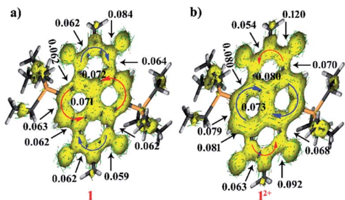
Fig. 6 AI CD isosurface plots of (a) 1 , and (b) 1 2+ . The induced ring current vectors are plotted on the AI CD isosurface to denote the diatropic and paratropic ring currents. The AI CD plots are plotted at an isosurface value of 0.05.
