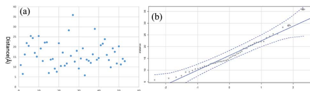
Fig. 7 The distribution of all the linkages: (a) Cα–Cα distance and (b) QQ plot.
