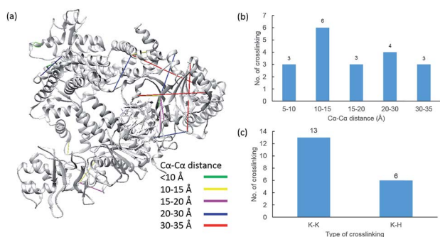
Fig. 8 Assessment of cross linkages with the Cpf1 3D structure: (a) cross-links mapped onto the crystal structures of Cpf1 (PDB entry 5ID6); (b) distribution of the Cα–Cα distance of the identified linkages; and (c) types of cross-linking sites identified from the pBVS cross-linked Cpf1 sample, with numbers indicated on top.
