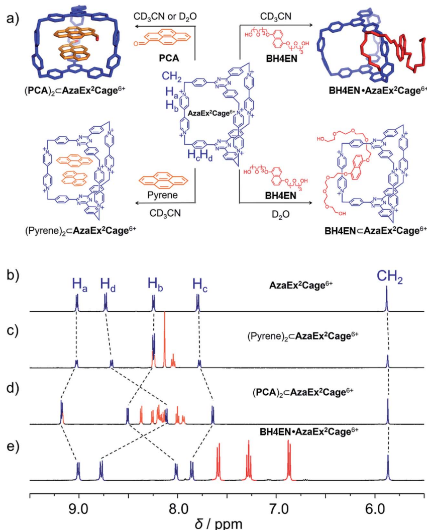
Fig. 1 (a) Schematic representation of the ability of AzaEx 2 Cage 6+ to recognize a variety of guests, including pyrene, PCA, and BH 4 EN. In the cases of pyrene and PCA, 2 : 1 complexes are formed, even though the ability of the cage to host the former guest is much weaker. In the case of BH 4 EN, the complex BH 4 EN·AzaEx 2 Cage 6+ forms in a peripheral and inclusion manner in CD 3 CN and D 2 O, respectively. 1 H NMR spectra of AzaEx 2 Cage·6PF 6 (500 MHz, 1.0 mM in CD 3 CN, 298 K) (b) before and after adding (c) pyrene (8.4 equiv.), (d) PCA (10.8 equiv.), and (e) BH 4 EN (11.4 equiv.). The resonances of the protons in AzaEx 2 Cage 6+ are labeled in the corresponding spectra. Addition of pyrene and PCA results in upfield shifts of the resonances of the phenylene residues (H c and H d ) in AzaEx 2 Cage 6+ , while the presence of BH 4 EN leads to upfield shifting of the resonances for the protons on BIPY 2+ (H a and H b ).
