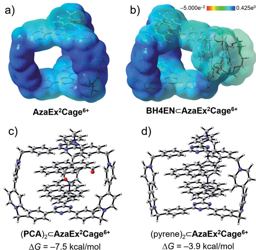
Fig. 8 Electrostatic potential maps for (a) \text{AzaEx}^2\text{Cage}^{6+} and (b) \text{BH4EN} \subset \text{AzaEx}^2\text{Cage}^{6+} obtained by using DFT calculations. Light-yellow and deep-blue colors in the maps represent negative and positive electrostatic potentials, respectively, demonstrating that the \text{BIPY}^{2+} units represent better \pi -electron acceptors on account of their stronger \pi -electron deficiency. DFT-optimized structures of (c) (\text{PCA})_2 \subset \text{AzaEx}^2\text{Cage}^{6+} and (d) (\text{pyrene})_2 \subset \text{AzaEx}^2\text{Cage}^{6+} . The free energy changes ( \Delta G ) for the formation of (\text{PCA})_2 \subset \text{AzaEx}^2\text{Cage}^{6+} and (\text{pyrene})_2 \subset \text{AzaEx}^2\text{Cage}^{6+} complexes are calculated to be -7.5 and -3.9 kcal mol -1 , respectively.
