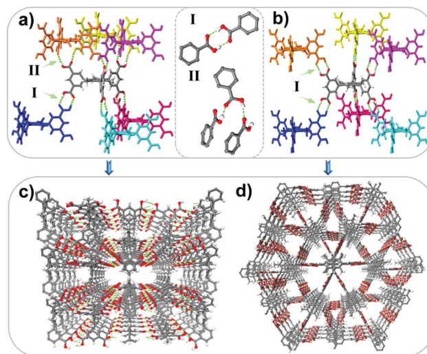
Fig. 1 Hydrogen-bonding interactions of JLU-SOF2 and JLU-SOF3 and their different intermolecular -COOH \cdots HOOC- hydrogen-bonding motifs (a and b); ball-and-stick models of JLU-SOF2 and JLU-SOF3 along the x-axis and z-axis, respectively (c and d).
