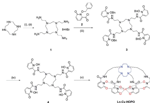
Scheme 1 Synthetic route of Ln-Cy-HOPO. (i) tosylaziridine, MeCN/benzene; (ii) AcOH/HBr; (iii) DIPEA, THF; (iv) AcOH/HCl; (v) LnCl 3 ·6H 2 O, pyridine, MeOH, 55 °C, 8 h.
