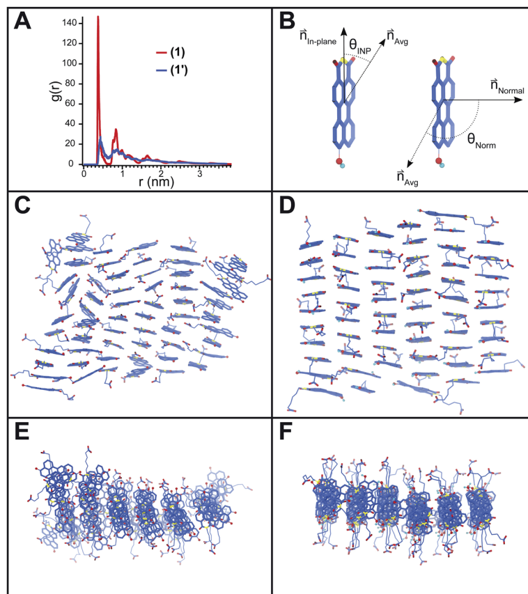
Fig. 5 Snapshots of MD simulations on pre-assembled PMI nanoscale ribbons. (A) Radial distribution function of the PMI center to center distance for both 1 and 1' . (B) Schematic of the two vectors ( n_{\text{in-plane}} , n_{\text{avg}} ) used to describe the rotational order of PMI assemblies. (C) Top view of 1' after equilibrium is reached. (D) Top view of 1 after equilibrium is reached. (E) Side view of 1' . (F) Side view of 1 . Explicit water molecules used in the simulations are omitted from snapshots for clarity.
