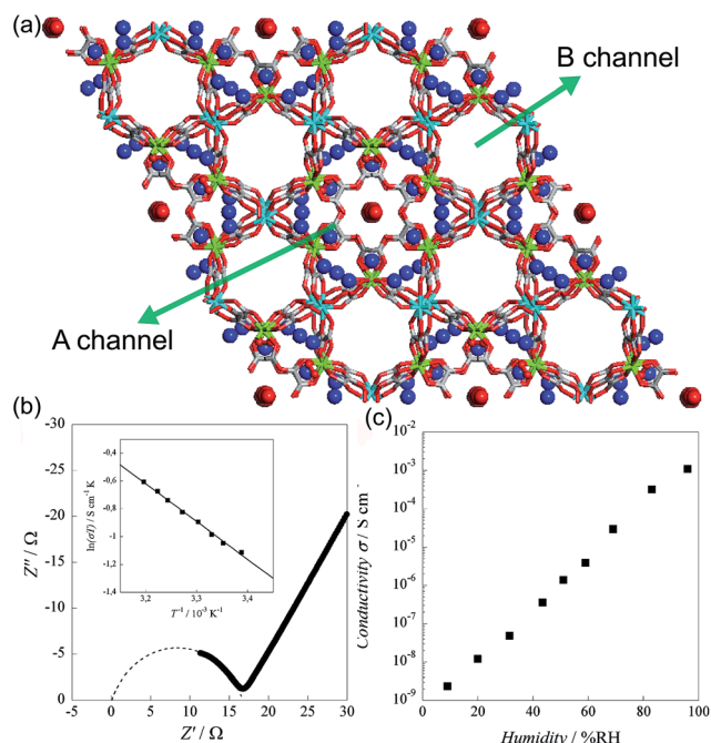
Fig. 15 (a) Structure of (\text{NH}_4)_4[\text{MnCr}_2(\text{ox})_6]\cdot 4\text{H}_2\text{O} . \text{NH}_4^+ counterion and \text{H}_2\text{O} guest molecules are represented as a sphere. Red, green, gray, cyan, and blue correspond to oxygen, chromium, carbon, manganese, and nitrogen atoms, respectively. (b) Cole–Cole semi-circle plot at 295 K and 96% RH. (c) RH dependence of \sigma for (\text{NH}_4)_4[\text{MnCr}_2(\text{ox})_6]\cdot 4\text{H}_2\text{O} at 295 K. Reproduced from ref. 72 with permission from American Chemical Society, Copyright 2011.
