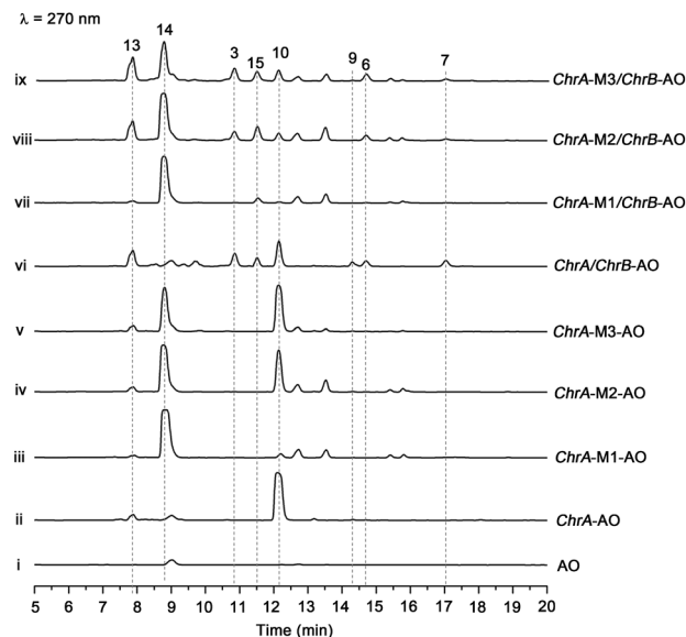
Fig. 5 Co-expression of KR-mutated ChrA and ChrB in A. oryzae (AO). HPLC traces for metabolites produced by AO ((i), as a blank reference), the transformants [with ChrA ((ii), ChrA -M1 for K 1829 D ((iii), ChrA -M2 for S 1853 A ((iv), and ChrA -M3 for Y 1866 A ((v)), and the co-transformants with ChrA and ChrB ((vi), ChrA -M1 and ChrB ((vii), ChrA -M2 and ChrB ((viii), and ChrA -M3 and ChrB ((ix)).
