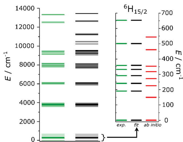
Fig. 2 Experimental (green) and fitted (black) energy level splitting. The inset is a zoom on the ground {}^6H_{15/2} term, where also the ab initio (red) energies are reported.
