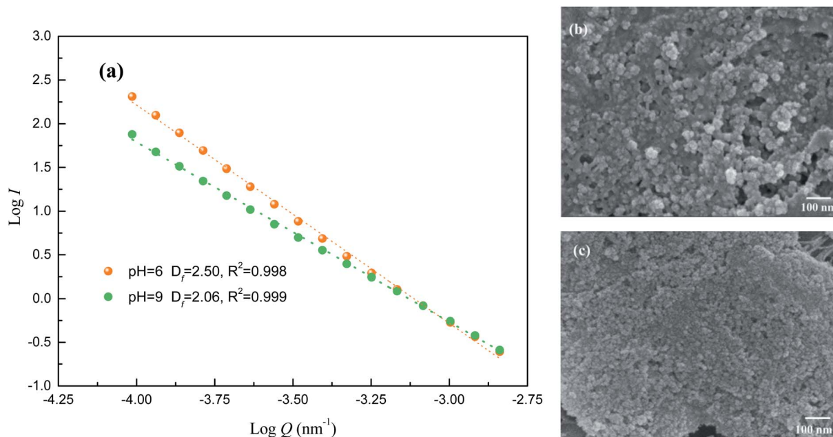
Fig. 7 Structure analysis of floc generated in acidic and alkaline conditions: (a) D_f of flocs; (b) SEM image of flocs at pH 9.0; (c) SEM image of flocs at pH 6.0.
