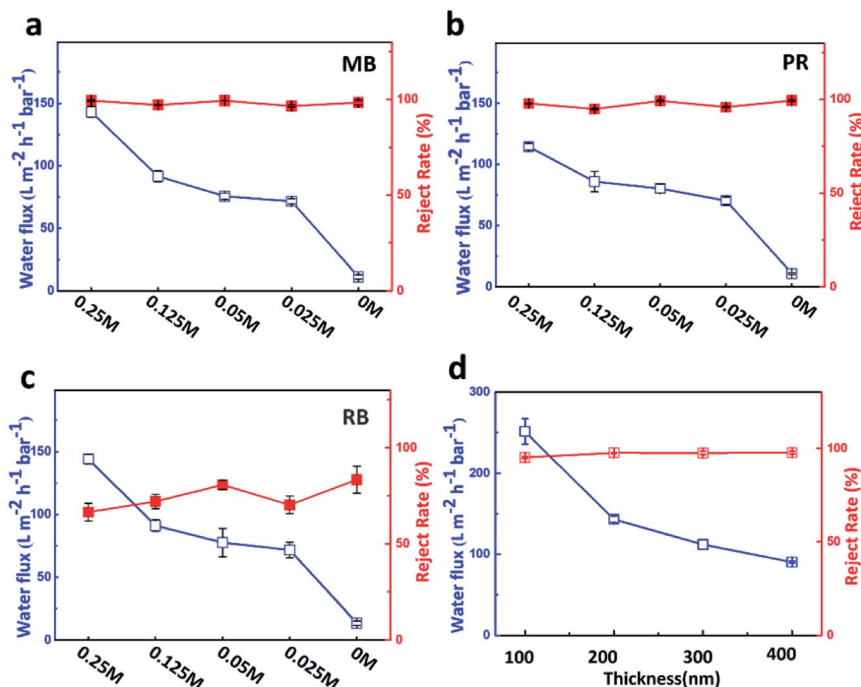
Fig. 4 Permeance and reject rate of (a) methylene blue, (b) pararosaniline and (c) rhodamine B ( 10 \text{ mg L}^{-1} ) by \text{GO}_{\text{HDA-Mg}^{2+}} membrane formed with different \text{Mg}^{2+} concentrations solutions. (d) Permeance and reject rate of methylene blue of \text{GO}_{\text{HDA-0.25Mg}^{2+}} membranes with different thickness.
