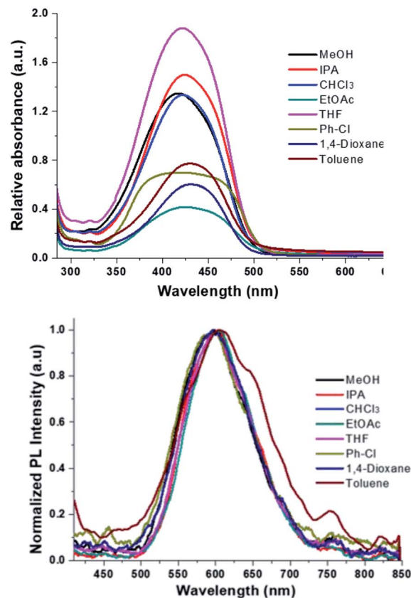
Fig. 9 HEMABM absorption and PL emissions spectra of the films (glass substrate) prepared with all solvents.
