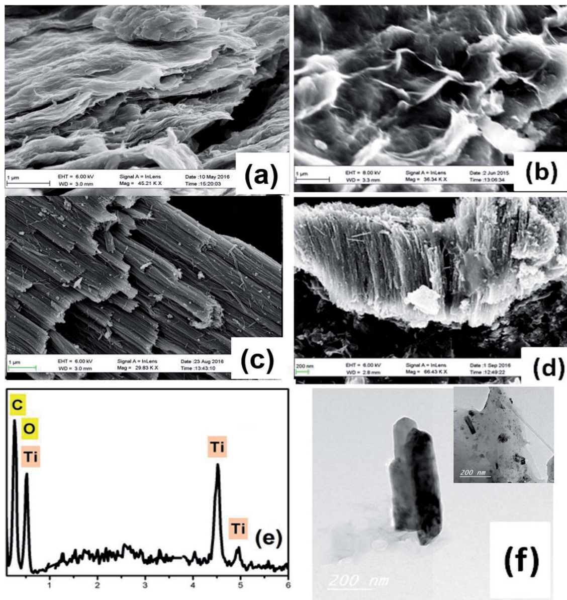
Fig. 1 FESEM images of (a) spongy GO, (b) FGO, (c) HTiO 2 , (d) FG-HTiO 2 , (e) EDS image and, (f) the TEM image of FG-HTiO 2 of the functionalize graphene-hydrogenated TiO 2 hybrid nanostructure.
