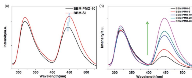
Fig. 5 Fluorescence emission spectra of (a) BBM-Si ( 10^{-6} M) and BBM-PMO-10 ( 5 \times 10^{-6} g mL ^{-1} ) in THF/ H_2O (3 : 7 v/v); (b) BBM-PMOs in THF/ H_2O (3 : 7 v/v, 5 \times 10^{-6} g mL ^{-1} ), from bottom to top are BBM-PMO-2, BBM-PMO-5, BBM-PMO-10, BBM-PMO-20 and BBM-PMO-40.
