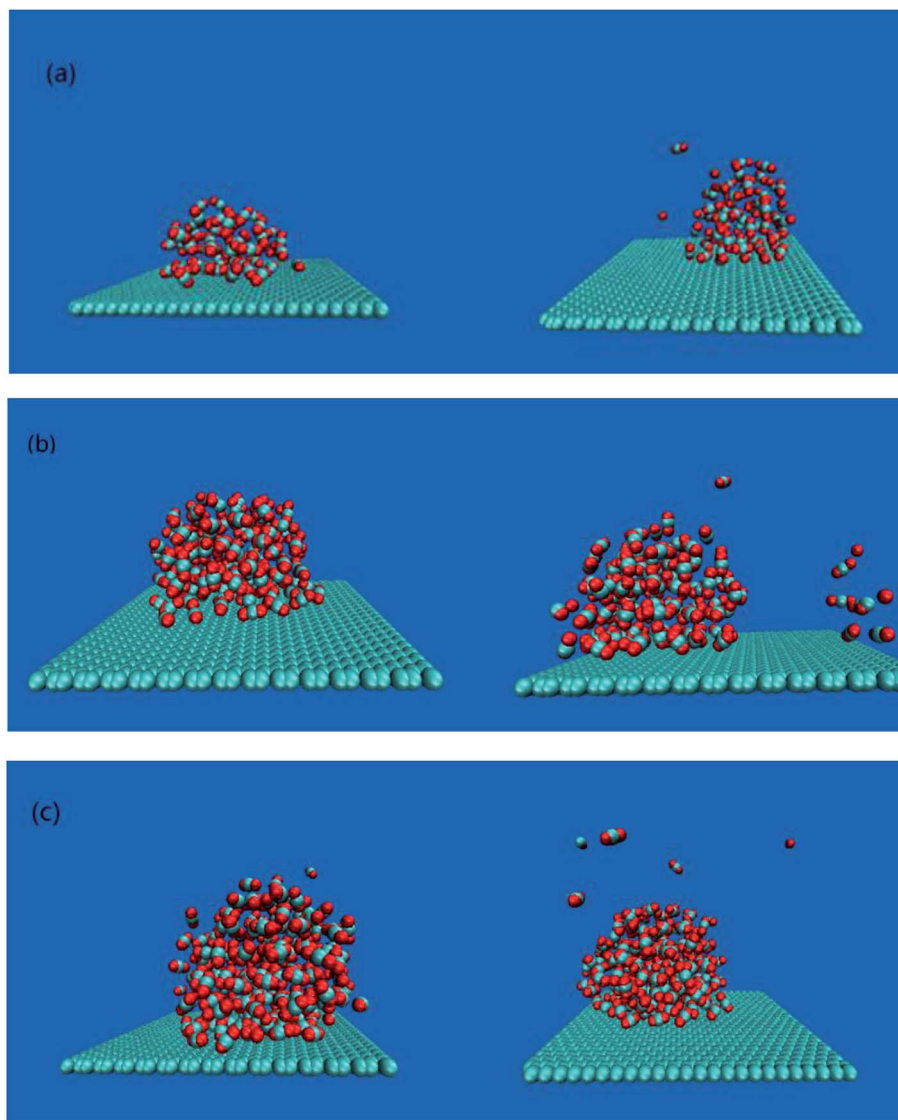
Fig. 2 Snapshot of bubbles under different systems. (a), (b) and (c) are bubbles formed by a system containing 60, 120 and 180 \text{CO}_2 molecules respectively, the left side is a bubble without an external electric field, and the right side is a bubble under an external electric field.
