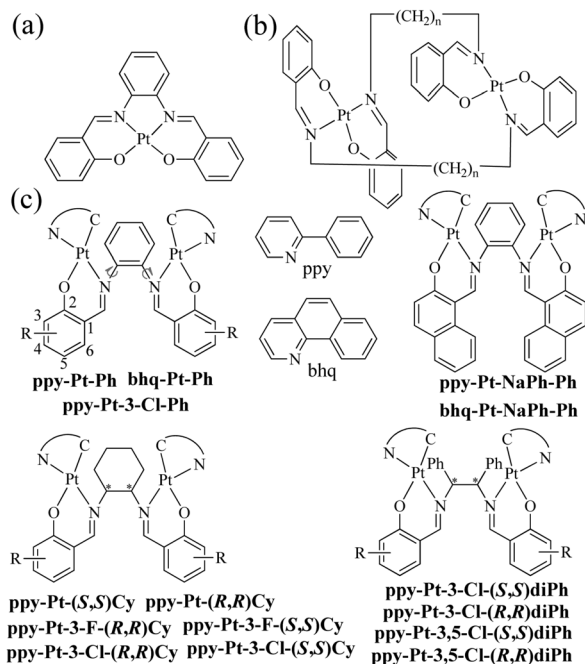
Scheme 1 Reported mononuclear Pt(Salen) complexes (a), reported binuclear Pt_2(Salen)_2 complexes (b), and stacked binuclear [(C^N)Pt(\mu-Salen)Pt(C^N)] complexes (c) in this work.
