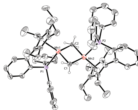
Fig. 5 Molecular structure of 4 with thermal ellipsoids at 30% probability. Hydrogen atoms, except that on carbon atoms C1 and C2, are omitted for clarity. Selected bond lengths [Å] and angles [°]: Mn(1)–C(1): 2.2249(18), Mn(1)–C(2): 2.308(2), Mn(1)–P(1): 2.7056(6), and C(1)–Mn(1)–C(2): 104.24(7).
