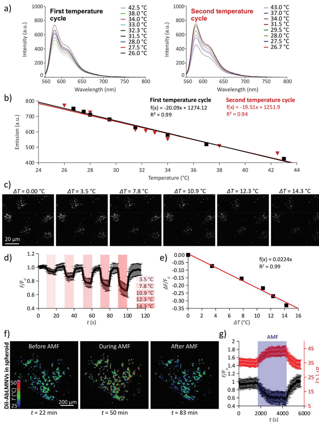
Fig. 6 Intraparticle temperature monitoring during AMF stimulation. (a) Thermosensitivity of fluorescence of the DiI dye in DMSO; fluorescence emission of DiI during two temperature cycles, shown in the left and right graphs, respectively. (b) Linear dependency between the DiI fluorescence emission peak (at \lambda = 583 nm) and the temperature during the two temperature cycles (shown in black and in red, respectively). (c) Fluorescence imaging of the DiI-labeled AbLMNVs during heating ( \Delta T_1 = 0.0 °C; \Delta T_2 = 3.5 °C; \Delta T_3 = 7.8 °C; \Delta T_4 = 10.9 °C; \Delta T_5 = 12.3 °C; and \Delta T_6 = 14.3 °C) induced by an infrared (IR) laser source. (d) Fluorescence intensity ( F/F_0 ) of the DiI-labeled AbLMNVs during heating. (e) Linear relation between \Delta F/F_0 and \Delta T in DiI-labeled AbLMNVs. (f) Temperature imaging of DiI-labeled AbLMNVs internalized into a GBM spheroid before, during, and after the AMF stimulation. (g) Graph reporting the F/F_0 and the \Delta T time course of DiI-AbLMNVs in GBM spheroids during AMF stimulation (the period of AMF exposure is highlighted in blue).
