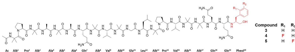
Fig. 3 Structures of the peptaibols, alamethicin F50 (3), ortho -F-phenol alamethicin F50 (4), and meta -F-phenol alamethicin F50 (5). The incorporation of the fluorinated derivatives of Phe at residue 20 via precursor-directed biosynthesis was monitored and optimized by in situ evaluation by droplet probe. The structures of these non-natural natural products were then verified by scaled up isolation and structure elucidation, 66 including Marfey's analysis, which confirmed incorporation of the L-enantiomers of F-Phe.
