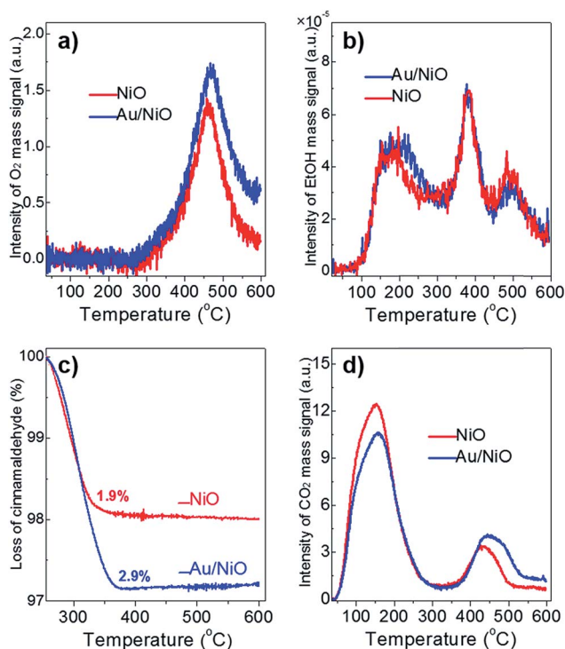
Fig. 2 (a) \text{O}_2 -TPD, (b) EtOH-TPD, and (c) TGA analysis of the chemisorbed cinnamaldehyde, and (d) \text{CO}_2 -TPD over the free NiO (red lines) and the Au/NiO composite (blue lines).
