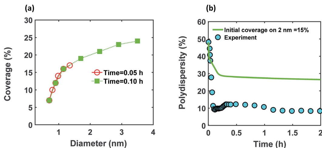
Fig. 5 (a) Model prediction of coverage vs. nanoparticle diameter at time = 0.05 and 0.10 h; (b) time evolution of polydispersity ( P(t) = \frac{\sigma(t)}{D_{ave}(t)} ). At time zero, the 2 nm nanoparticle population has 15% initial ligand coverage, while the initial coverage of smaller size population; 0.6 nm, is zero. Experimental conditions: 10 mM Pd(OAc) 2 in 1 : 1 pyridine/hexanol, TOP : Pd = 1, and T = 100^\circ\text{C} .
