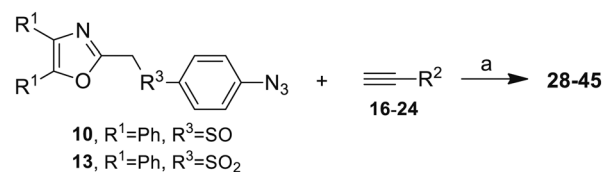
Scheme 2 Click reactions of azidophenylsulfoxides 10 and azidophenyl-sulfones 13 with selected arylalkynes 16–24 to give Group I triazoles 28–45 . a Reagents/conditions: CuSO 4 ·5H 2 O/Na ascorbate/THF–H 2 O (2 : 1).
