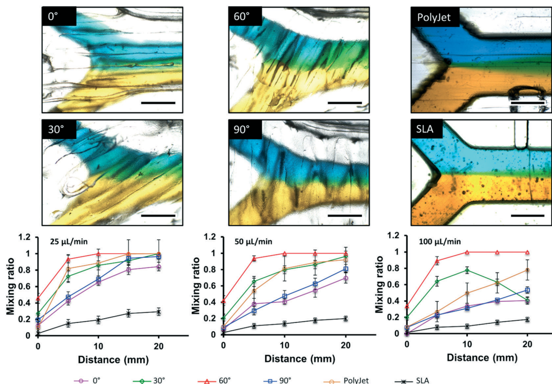
Fig. 2 Microscopic images of laminar flow within 500\ \mu\text{m} \times 500\ \mu\text{m} channels into 750\ \mu\text{m} \times 500\ \mu\text{m} channels, visualized with yellow and blue food dye at 25\ \mu\text{L}\ \text{min}^{-1} for FDM 0^\circ , 30^\circ , 60^\circ , and 90^\circ , PolyJet, and SLA, respectively. Plots of distance vs. mixing ratio, demonstrating diffusion through the laminar flow channel at 25, 50, and 100\ \mu\text{L}\ \text{min}^{-1} are also shown below the microscopic images. N = 3 , scale bar = 500\ \mu\text{m} . Reproduced from ref. 41 with permission.
