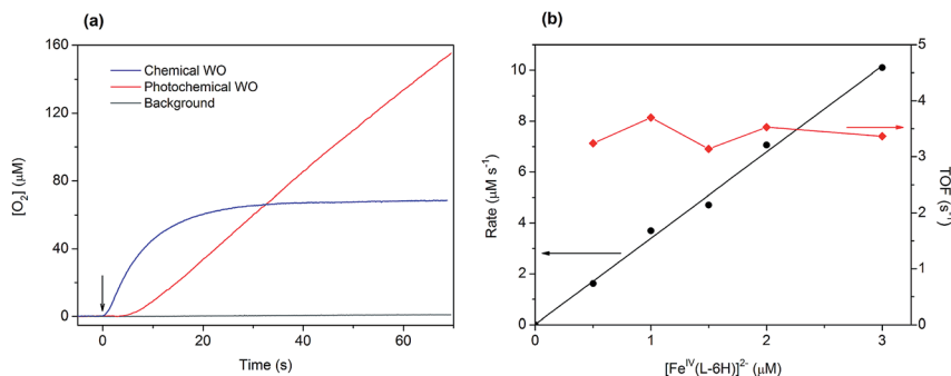
Fig. 3 (a) Traces of oxygen evolution obtained in photochemical (red trace: [\text{Fe}^{\text{IV}}(\text{L-6H})]^{2-} (1 \mu\text{M} ), [\text{Ru}(\text{bpy})_3]^{2+} (0.2 mM) and \text{S}_2\text{O}_8^{2-} (2 mM)) and chemical water oxidation experiments (blue trace: [\text{Fe}^{\text{IV}}(\text{L-6H})]^{2-} (1.5 \mu\text{M} ) and [\text{Ru}(\text{bpy})_3]^{3+} (1 mM)). Oxygen evolution in the absence of catalyst is given for comparison (grey trace: [\text{Ru}(\text{bpy})_3]^{2+} (0.2 mM) and \text{S}_2\text{O}_8^{2-} (2 mM)). The arrow indicates the beginning of the reaction (the start of illumination or addition of the oxidant, respectively). (b) Initial water oxidation rates (circles) and TOF (diamonds) as a function of the catalyst concentration for chemical water oxidation using [\text{Ru}(\text{bpy})_3]^{3+} (1 mM).
