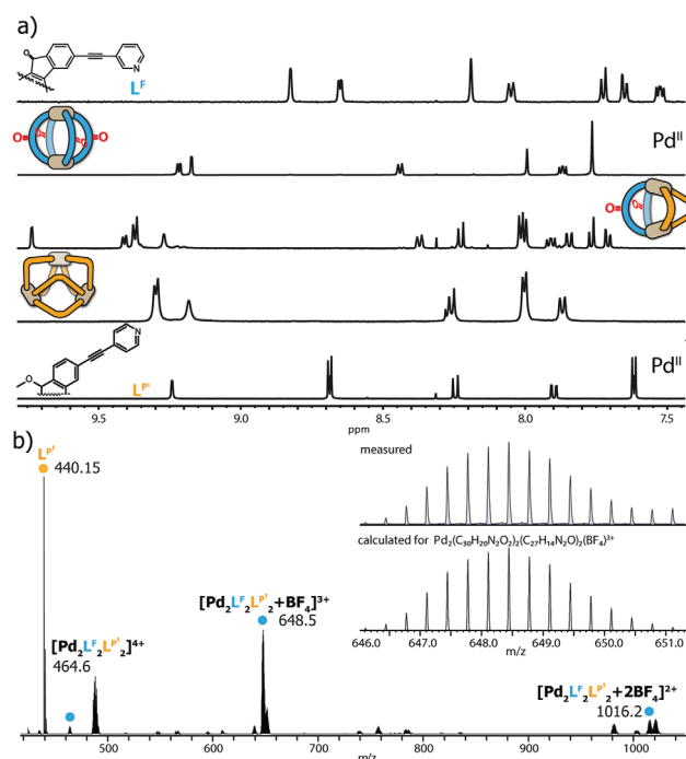
Fig. 2 (a) ^1H NMR spectra of L^F , homoleptic [Pd_2L^F_4]^{4+} , heteroleptic [Pd_2L^FL^P_2]^{4+} , homoleptic [Pd_3L^P_6]^{6+} and L^P (from top to bottom, 500 MHz, 298 K, DMSO- d_6 ); (b) ESI mass spectrum of heteroleptic [Pd_2L^FL^P_2]^{4+} , including BF_4^- adducts.
