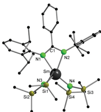
Fig. 2 Molecular structure of 2 in the solid-state. Hydrogen atoms and solvent molecules are omitted for clarity. Selected bond lengths [Å], angles [°]: \text{Sm-N1} 2.421(3), \text{Sm-N2} 2.415(3), \text{Sm-N3} 2.306(3), \text{Sm-N4} 2.297(3), \text{Si1-N3} 1.727(3), \text{Si2-N3} 1.705(4), \text{Si3-N4} 1.715(3), \text{Si4-N4} 1.728(4), \text{N1-C1} 1.330(5), \text{N2-C1} 1.354(5); \text{N1-Sm-N2} 55.56(11), \text{N3-Sm-N4} 121.49(13), \text{N1-C1-N2} 114.2(4).
