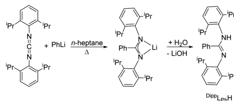
Scheme 3 Synthesis of D^{iPr}_2L_{PhH} . 55
