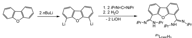
Scheme 2 Synthesis of iPr_2L_{DBFH_2} . 49
