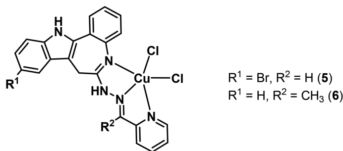
Chart 3 Paullone-derived copper(II) complexes used in this study. 15,25
