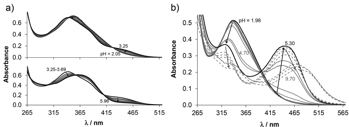
Fig. 4 UV-vis spectra recorded for (a) \text{HL}^3 and (b) complex 3 at various pH values in 30–70% (w/w) DMSO–water solvent mixture. \{c_{\text{ligand}} = c_{\text{complex}} = 12.5 \mu\text{M}; T = 298 \text{ K}; I = 0.10 \text{ M (KCl)}; l = 2 \text{ cm}\} .
