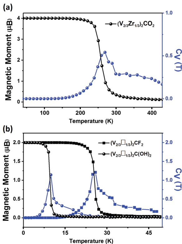
Fig. 4 Variation of the total magnetic momentum (per unit cell) of (a) (\text{V}_{2/3}\text{Zr}_{1/3})_2\text{CO}_2 (b) (\text{V}_{2/3}\square_{1/3})_2\text{CF}_2 and (\text{V}_{2/3}\square_{1/3})_2\text{C(OH)}_2 with respect to the temperature. Corresponding specific heats C_V are shown in blue.
