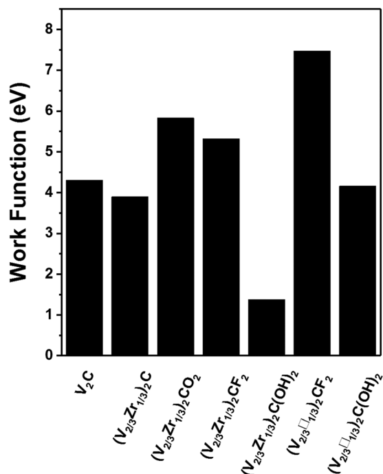
Fig. 5 Work functions of \text{V}_2\text{C} , pristine (\text{V}_{2/3}\text{Zr}_{1/3})_2\text{C} , bimetallic (\text{V}_{2/3}\text{Zr}_{1/3})_2\text{CX}_2 and vacancy-ordered (\text{V}_{2/3}\square_{1/3})_2\text{CX}_2 MXenes.
