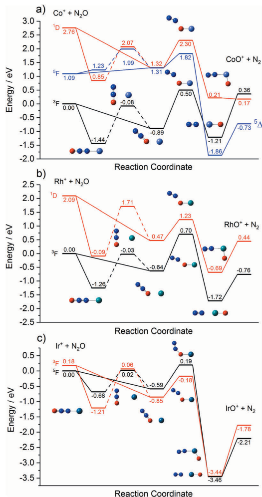
Fig. 2 Potential energy profiles for M^+ + N_2O insertion ( M = (a) Co, (b) Rh, and (c) Ir). Black and red (blue in (a) ) solid lines refer to ground and excited states of the metal cations, respectively. In each case, M^+ + N_2O can form an N- or an O-bound complex, represented here as two pathways for each multiplicity (two lines from ground state cation and two lines from excited cation). Dashed lines represent the barrier to internal rotation, as the insertion reaction could begin from the N-bound complex, but also from the O-bound complex.
