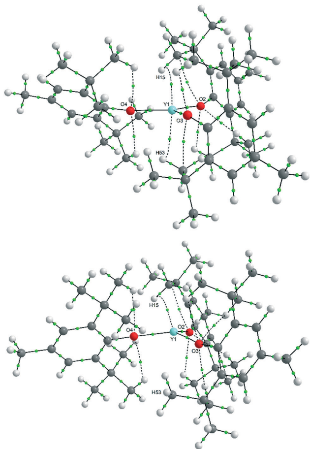
Fig. 6 QTAIM plot of bond paths with BCPs (green) for planar (top) and pyramidal \text{Y}(\text{OAr})_3 , (bottom) conformers showing the presence of multiple weak \text{O}\cdots\text{H} interactions in addition to the \text{Y}\cdots\text{H} interactions ( \rho cut-off = 0.015). Weak ( \rho < 0.05 ) bond paths are shown as dashed lines. NB: numbering scheme differs to crystal structure.
