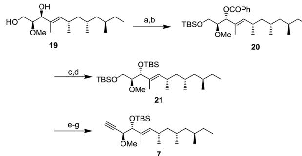
Scheme 4 Synthesis of alkyne 7 ; (a) TBSCl, imidazole, \text{CH}_2\text{Cl}_2 , r.t., 2 h, 81%; (b) \text{PhCOOH} , DEAD, \text{PPh}_3 , THF, r.t., 15 h, 95%; (c) \text{K}_2\text{CO}_3 , MeOH, r.t., 12 h; (d) TBSOTf, 2,6-lutidine, \text{CH}_2\text{Cl}_2 , -78 °C, 2 h, 98% (2 steps); (e) PPTS, EtOH, r.t., 16 h, 80%; (f) DMP, \text{CH}_2\text{Cl}_2 , r.t., 2 h; and (g) dimethyl(1-diazo-2-oxopropyl)phosphonate, \text{K}_2\text{CO}_3 , MeOH, r.t., 18 h, 58% (2 steps).
