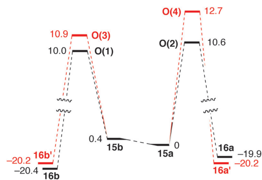
Fig. 4 Reaction pathway for H - transfer in mechanism O . Relative Gibbs free energies are in kcal mol -1 (reprinted with permission from ref. 88. Copyright 2018 American Chemical Society).
