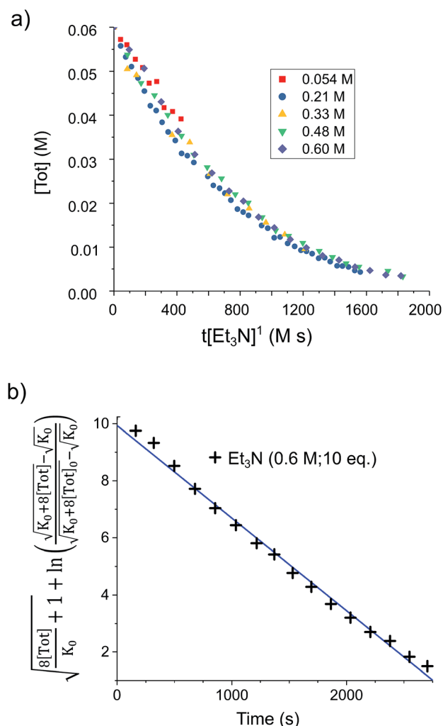
Fig. 3 (a) Solutions of 1 (0.03 mmol) in d_8 -toluene (0.5 mL) under H_2 (4 bar) containing various base concentrations were prepared. When the stannylenic concentration, [Tot] , is plotted against the normalised timescale t \cdot [Et_3N]^1 , all traces overlap, confirming the order in base to be one. (b) Linearised rate data for a similar solution of 1 (0.03 mmol) in d_8 -toluene (0.5 mL) under H_2 (4 bar) containing Et_3N (0.6 M; 10 eq.).
