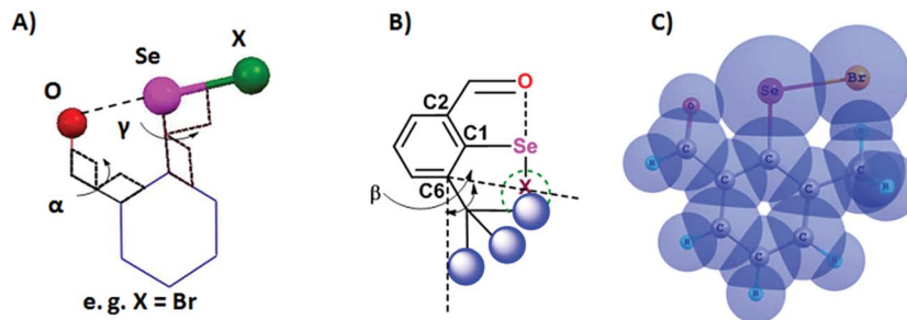
Fig. 4 (A) Illustration of the O\cdots Se-X interaction. (B) Illustration of the cone angle, (C) space-filling model showing the steric collision of methyl hydrogen with bromine (CH_3)\cdots(Br) .
