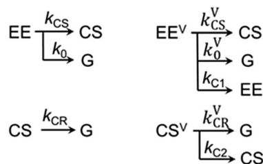
Fig. 3 Kinetic scheme used to describe the three-pulse data. EE represents the acceptor localized excited electronic state and G represents the ground electronic state. The superscript "V" labels the vibrationally excited electronic states. CS is the charge separated electronic state.
