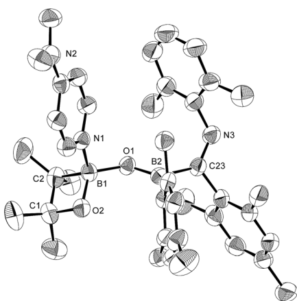
Fig. 7 Molecular structure of 10 (thermal ellipsoids set at 50% probability; co-crystallized molecules of toluene and hydrogen atoms omitted for clarity). Selected bond distances (Å), angles ( ^\circ ) and dihedral angles ( ^\circ ): B1–O1 1.470(4), B1–O2 1.465(4), B1–C2 1.628(5), B1–N1 1.612(4), O1–B2 1.330(4), B2–C23 1.641(5), C23–N3 1.295(4), O2–B1–O1 117.0(3), O2–B1–N1 110.6(2), O1–B1–N1 105.2(2), O2–B1–C2 91.6(2), O1–B1–C2 118.4(3), N1–B1–C2 113.9(3), B1–O2–C1 91.2(2), B1–O1–B2 128.6(3), O1–B2–C23 118.1(3), B2–C23–N3 127.9(3), B1–O1–B2–C23 176.5(3), O1–B2–C23–N3 63.4(4).
