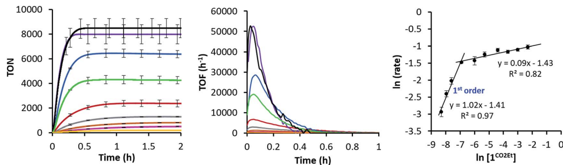
Fig. 5 (Left) Dependence of the H_2 evolution with the concentration of 1^{CO_2Et} (100 \mu M , yellow; 50 \mu M , pink; 25 \mu M , orange; 12.5 \mu M , grey; 5 \mu M , red; 2.5 \mu M , green; 1 \mu M , blue; 0.5 \mu M , purple; 0.25 \mu M , black). (Middle) On-line H_2 evolved traces and rates vs. time at different concentrations of 1^{CO_2Et} (0.25–100 \mu M ). Conditions: PS_{Ir}^+ (150 \mu M ) in CH_3CN : H_2O : Et_3N (4 : 6 : 0.2 mL) irradiated ( \lambda = 447 nm) at 25 ^\circ C . (Right) Logarithmic plot of catalytic rate as a function of 1^{CO_2Et} concentration.
