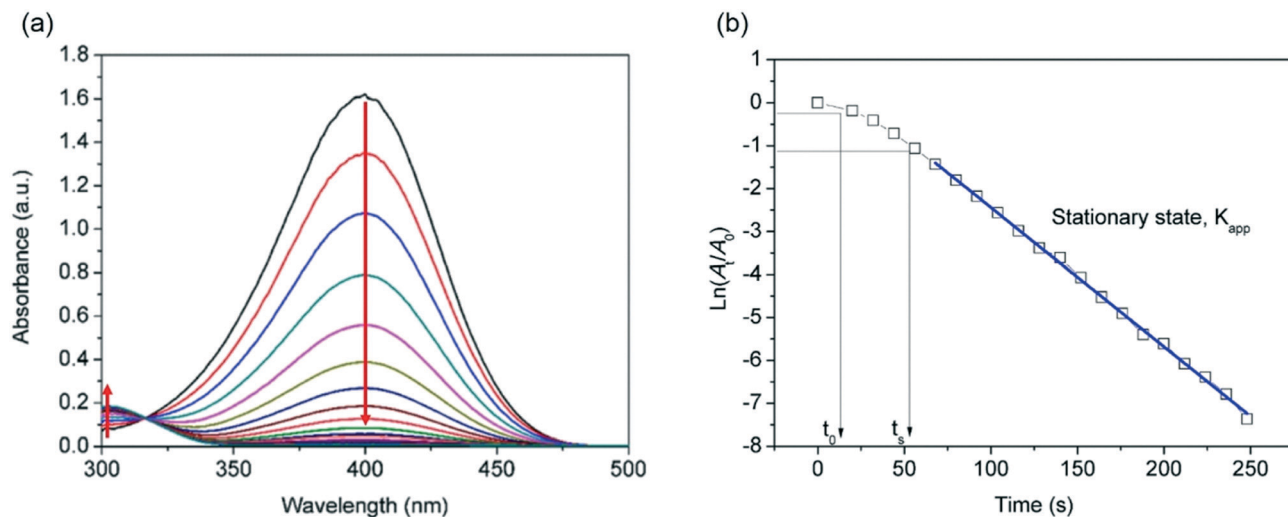
Fig. 12 Reduction of 4-nitrophenol by sodium borohydride by 2.24 \times 10^{-5} g L -1 silver nanoparticles. (a) UV-vis absorption spectra of the solution as a function of time. (b) Kinetic analysis of the system after the induction period.
