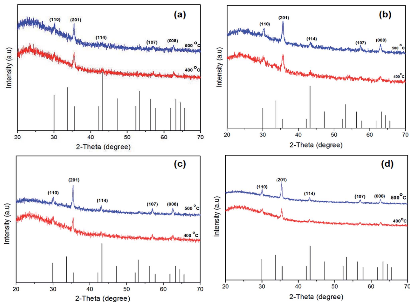
Fig. 3 Powder X-ray diffraction (p-XRD) patterns of the iron sulfide thin films obtained by spin coating [Fe(S 2 COMe) 3 ] (a), [Fe(S 2 COEt) 3 ] (b), [Fe(S 2 CO i Pr) 3 ] (c) and [Fe(S 2 CO n Pr) 3 ] (d) followed by annealing under nitrogen at 400–500 °C for 60 min. The black sticks represent hexagonal troilite phase (FeS). (ICDD: 01-075-2165).
