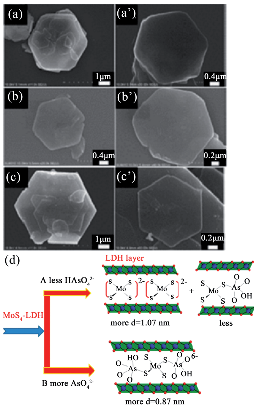
Fig. 6 SEM images of the samples after \text{MoS}_4\text{-LDH} adsorption with (a and a') 10 ppm \text{As}(\text{iii}) , (b and b') 300 ppm \text{As}(\text{iii}) and (c and c') 10 ppm \text{As}(\text{v}) ; (d) a scheme showing the dominant phases and possible binding modes of \text{MoS}_4^{2-} with \text{HAsO}_4^{2-} in the LDH gallery (adapted with permission from ref. 89).
