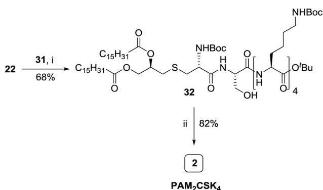
Scheme 4 Synthesis of PAM_2CSK_4 . Conditions: (i) H-[Lys(Boc)] 4 -O'Bu, EDCI, HOBT, Et 3 N, DMF, 6 h. (ii) HCl, dioxane, 2 h.
