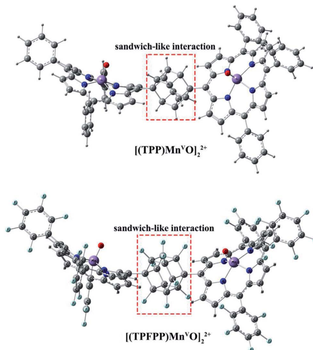
Fig. 1 Gas phase DFT optimized structure of the [(\text{TPP})\text{Mn}^{\text{VO}}\text{O}_2]^{2+} and [(\text{TPFPP})\text{Mn}^{\text{VO}}\text{O}_2]^{2+} .
