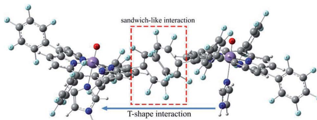
Fig. 2 Gas phase DFT optimized structure of the [(\text{TPFPP})(\text{ImH})\text{Mn}^{\text{VO}}\text{O}_2]^{2+} .
