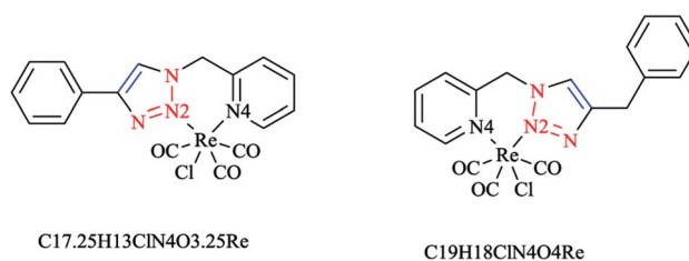
\text{C}_{19}\text{H}_{18}\text{ClN}_4\text{O}_4\text{Re}
