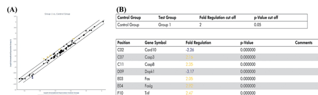
Fig. 4 MiR-122 affected various apoptosis pathway. (A) H9c2 cells were transfected with miR-122 mimics or NC vector, extracted by RNeasy ® mini kit, and reversed by RT 2 first strand kit followed by real-time fluorescent quantitative PCR. The normalized expressions of every gene on the array between miR-122 mimics (group 1) and NC group (control group) were compared and presented as scatter plot. The central line indicated unchanged gene expression. The dotted lines indicate the selected fold regulation threshold. Data points beyond the dotted lines in the upper left and lower right sections meet the selected fold regulation threshold. (B) The differentially expressed genes are listed with name and fold regulation. Fold-regulation represents fold-change results in a biologically meaningful way. Fold-change ( 2^{(-\Delta\Delta CT)} ) is the normalized gene expression ( 2^{(-\Delta\Delta CT)} ) in the test sample divided the normalized gene expression ( 2^{(-\Delta\Delta CT)} ) in the control sample (see ESI † data sheet for more details).
