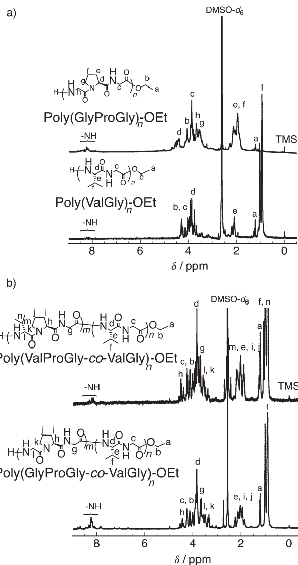
Fig. 2 ^1\text{H} NMR spectra of (a) poly(GlyProGly) and poly(ValGly) and (b) poly(ValProGly-co-ValGly) and poly(GlyProGly-co-ValGly), in \text{DMSO}-d_6 /TFA- d (5/1).
