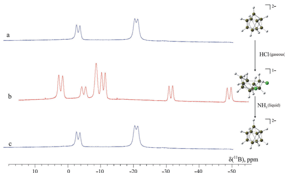
Fig. 2 ^{11}\text{B} NMR spectra of the \text{CD}_3\text{CN} solutions of the initial [\text{closo-B}_9\text{H}_9]^{2-} (a), the chlorine-containing derivative [\text{arachno-B}_9\text{H}_{12-4,8}\text{Cl}_2]^- (b) and the product of its reaction with liquid ammonia (c).
