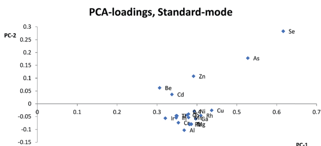
Fig. 5 Weighted PCA loadings according to explained variance including all matrixes in standard-mode, based on centered \ln(x) transformed data for ^9\text{Be} , ^{24}\text{Mg} , ^{27}\text{Al} , ^{49}\text{Ti} , ^{51}\text{V} , ^{53}\text{Cr} , ^{55}\text{Mn} , ^{59}\text{Co} , ^{61}\text{Ni} , ^{65}\text{Cu} , ^{67}\text{Zn} , ^{69}\text{Ga} , ^{75}\text{As} , ^{82}\text{Se} , ^{89}\text{Y} , ^{103}\text{Rh} , ^{111}\text{Cd} , ^{115}\text{In} , ^{193}\text{Ir} , ^{205}\text{Tl} , ^{208}\text{Pb} .
